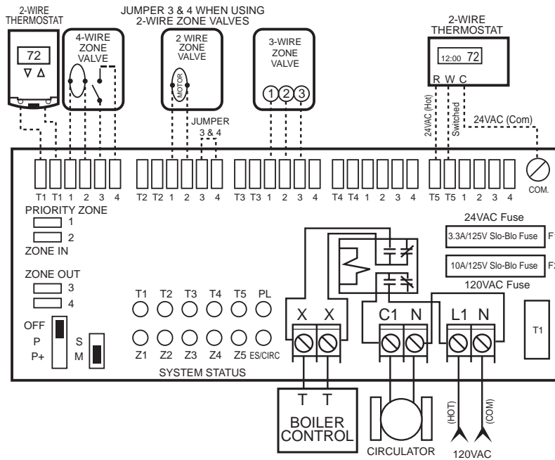
Figure 1 Typical Wiring.
