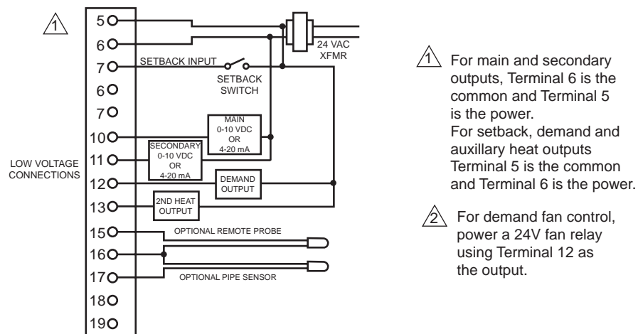
Figure 1 Typical Wiring for Proportional Control.
