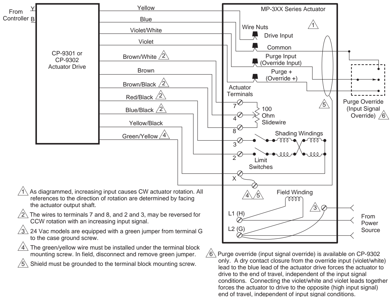
Figure 3 Proportional Electric Control, CP-930X.
