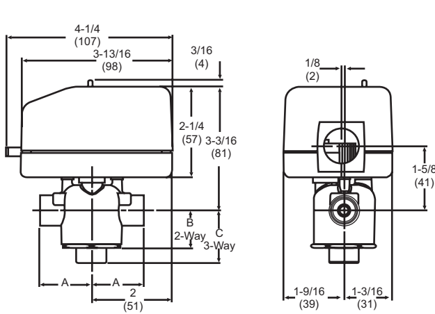
Figure 1 Modulating Non-Spring Return Valve.
