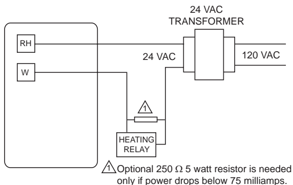
Figure 1 T201 Wiring to Heating System With Single Transformer.
