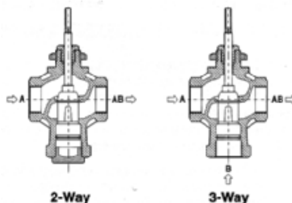
Figure 1 Valve Body Types.
