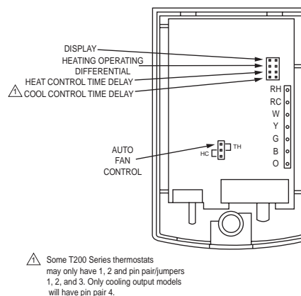
Figure 6 Terminal Identification.
