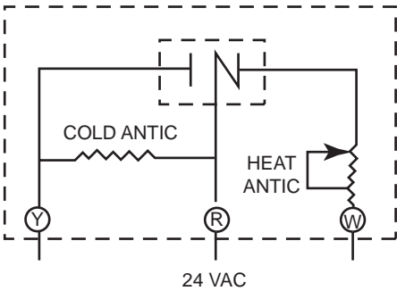
Figure 1 Heat/Cool Thermostats 31-100 and 31-102.
