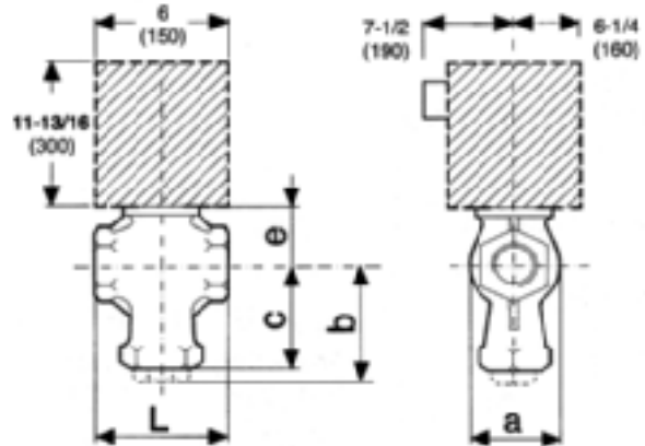
Figure 5 Dimensions.
