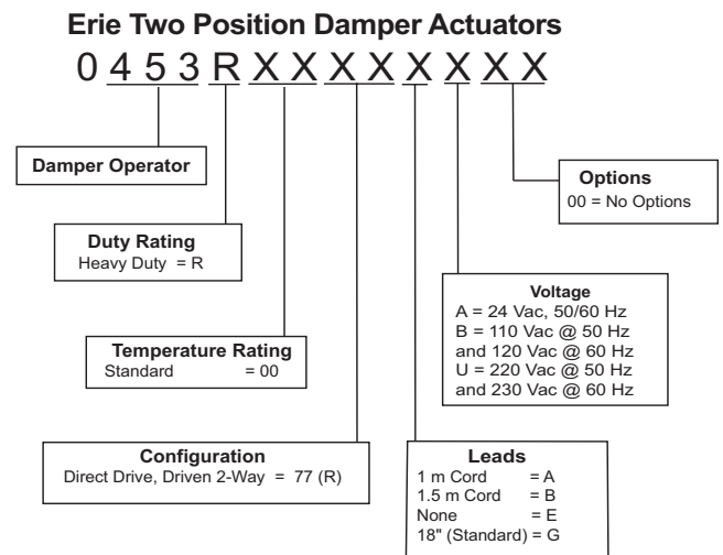
Figure 1 Selection Chart.
