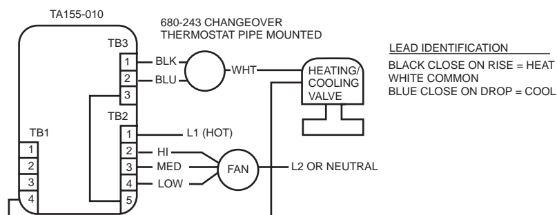
Figure 1 Typical Wiring.
