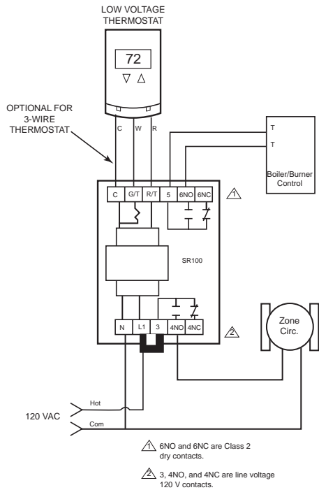
Figure 1 SR100 Relay Typical Wiring.
