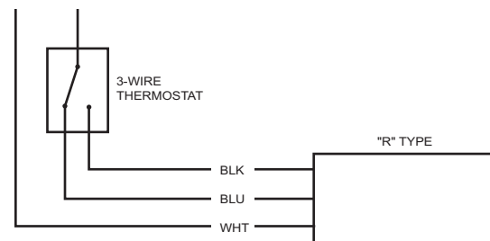
Figure 2 Wiring with 3-Wire Thermostat (18" Leads).
