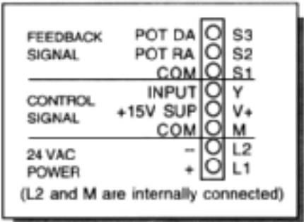
Figure 2 VAP100ANS Wiring.
