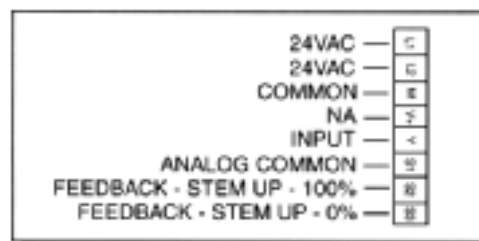
Figure 1 VAP270 Wiring Diagram.
