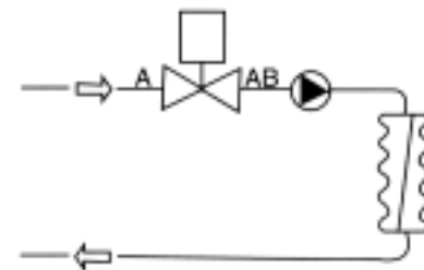
Figure 2 Two-Way Flow Direction.
