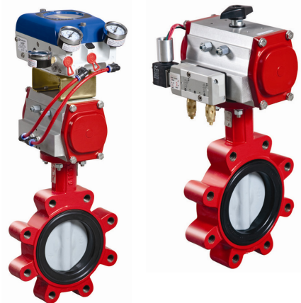
Two-Way, Industrial-Grade, Spring-Return, V-919x Series High-Pressure Pneumatically Actuated, Standard-Pressure, Standard-Temperature Butterfly Valve Assemblies
