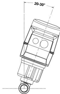
Horizontal mounting
