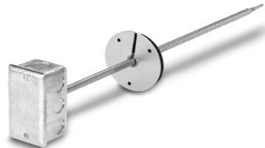
Figure 3. Duct (Single Point) Temperature Sensor (535-741-18 Shown with AQM2000 Accessory).
